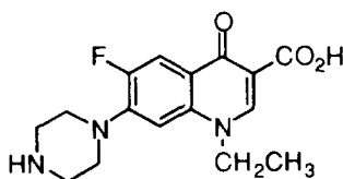
norfloxacin
