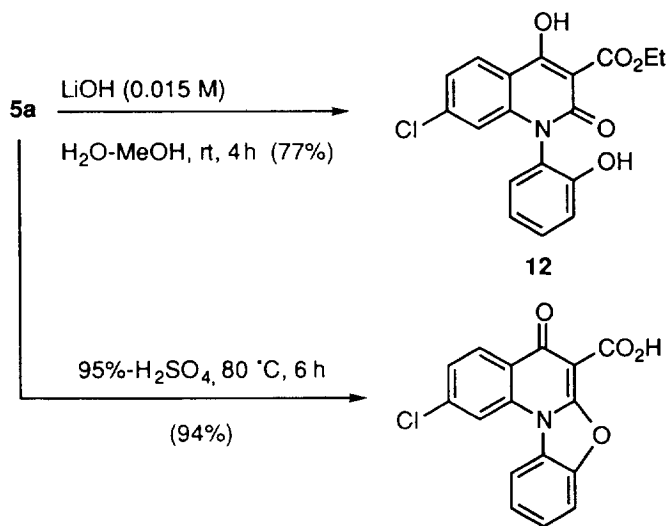
Scheme 7
