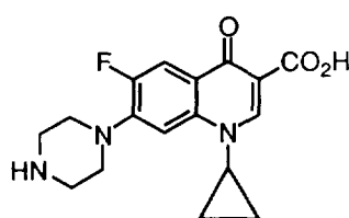
ciprofloxacin
